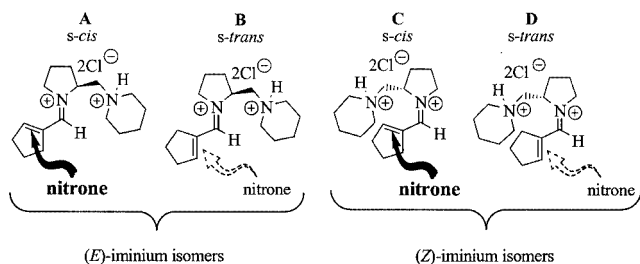
Figure 4. Potential reactive iminium ion intermediates A–D from catalyst 15 and aldehyde 1A ; as described by the arrows, \alpha -Si, \beta -Re attack on the \alpha,\beta -unsaturated iminium ion derivative gives the major enantiomer of the product obtained; filled arrows indicate attack from the front, and the unfilled ones attack from the back
