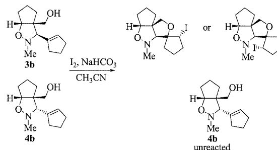
Scheme 4. Iodoetherification of a mixture of the reduced major cycloadduct 3b and the minor one 4b
