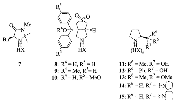
Figure 1. Organocatalysts for use in 1,3-dipolar cycloadditions of nitrones 2a–g with either aldehyde 1A or 1B
