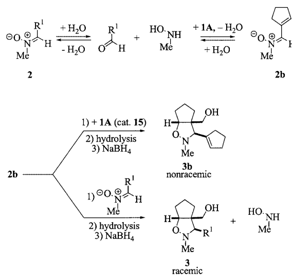
Scheme 3. Proposed competing reactions furnishing either nonracemic 3b as a by-product or one of the cycloadducts 3a–e as a racemate
