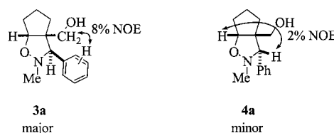
Figure 2. NOE observed in the major and minor diastereomer 3a and 4a , respectively
