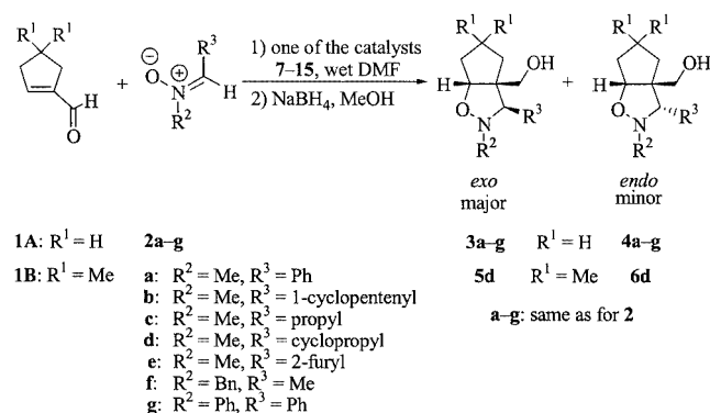
Scheme 1. The organocatalyzed reaction of either aldehyde 1A or 1B with various nitrones 2a–g
