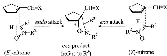
Figure 3. Origin of diastereoselectivity in the reactions of the nitrones 2a–g with the reactive intermediate from cyclopentenecarboxaldehyde 1A and catalyst 15 ; the definition of exo and endo attack is related to the \alpha,\beta -unsaturated system
