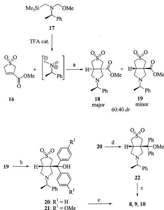
Scheme 2. Preparation of the potential organocatalysts 8–10 ; reagents and conditions: a) CH 2 Cl 2 , trifluoroacetic acid (cat.), 0 \rightarrow 20 ^{\circ}\text{C} , 94%; b) (i) PhMgBr or p -MeOC 6 H 4 MgBr, THF, (ii) water, 62%; c) (i) 1-chloroethyl chloroformate, 1,8-bis(dimethylamino)-naphthalene, ClCH 2 CH 2 Cl, reflux, (ii) MeOH, reflux, 65–96% overall yield; d) (i) NaH, MeI, THF, (ii) water, 88%
