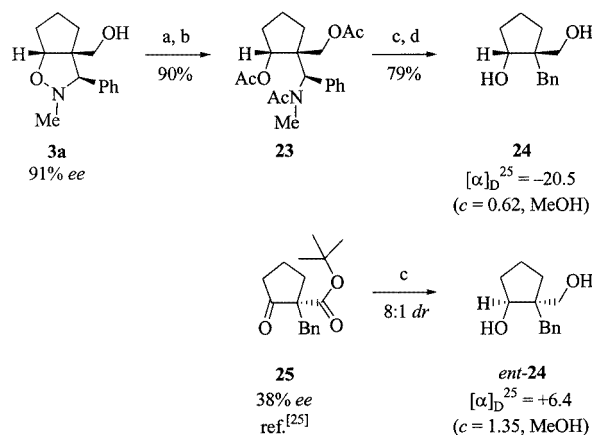
Scheme 5. Preparation of diol 24 and the enantiomer ent - 24 from compound 3a and 25 , respectively; reagents and conditions: a) \text{Pd}(\text{OH})_2 , HCl, MeOH, \text{H}_2 ; b) AcCl, pyridine, \text{CH}_2\text{Cl}_2 ; c) (i) \text{LiAlH}_4 , THF, (ii) water; d) Pd/C, \text{H}_2 , MeOH
